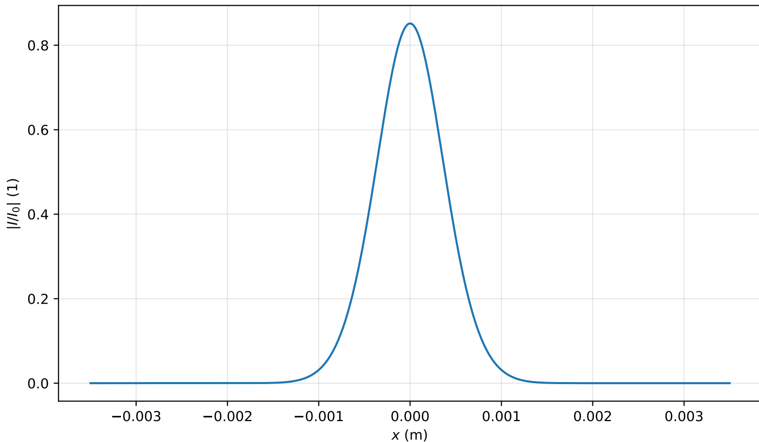
Intensity profile I(x, y = 0, z = 1.115m)/I_0 , P_{in}=0.2P_{cr} , artificial time
